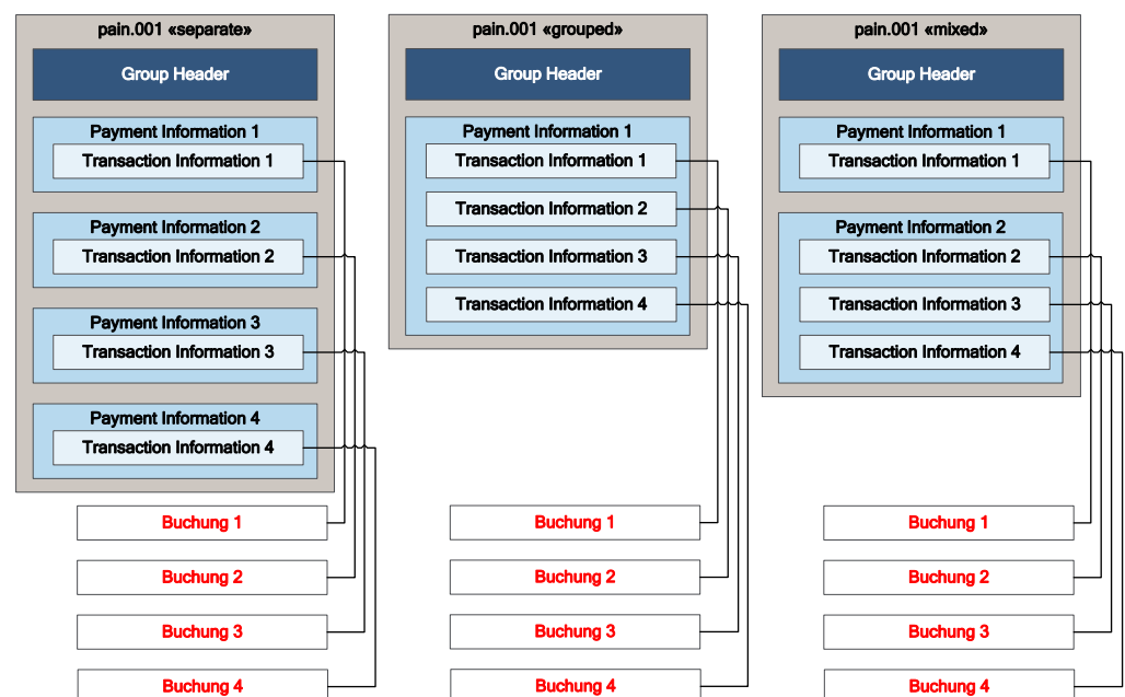
Figure 8: Batch Booking "FALSE"
