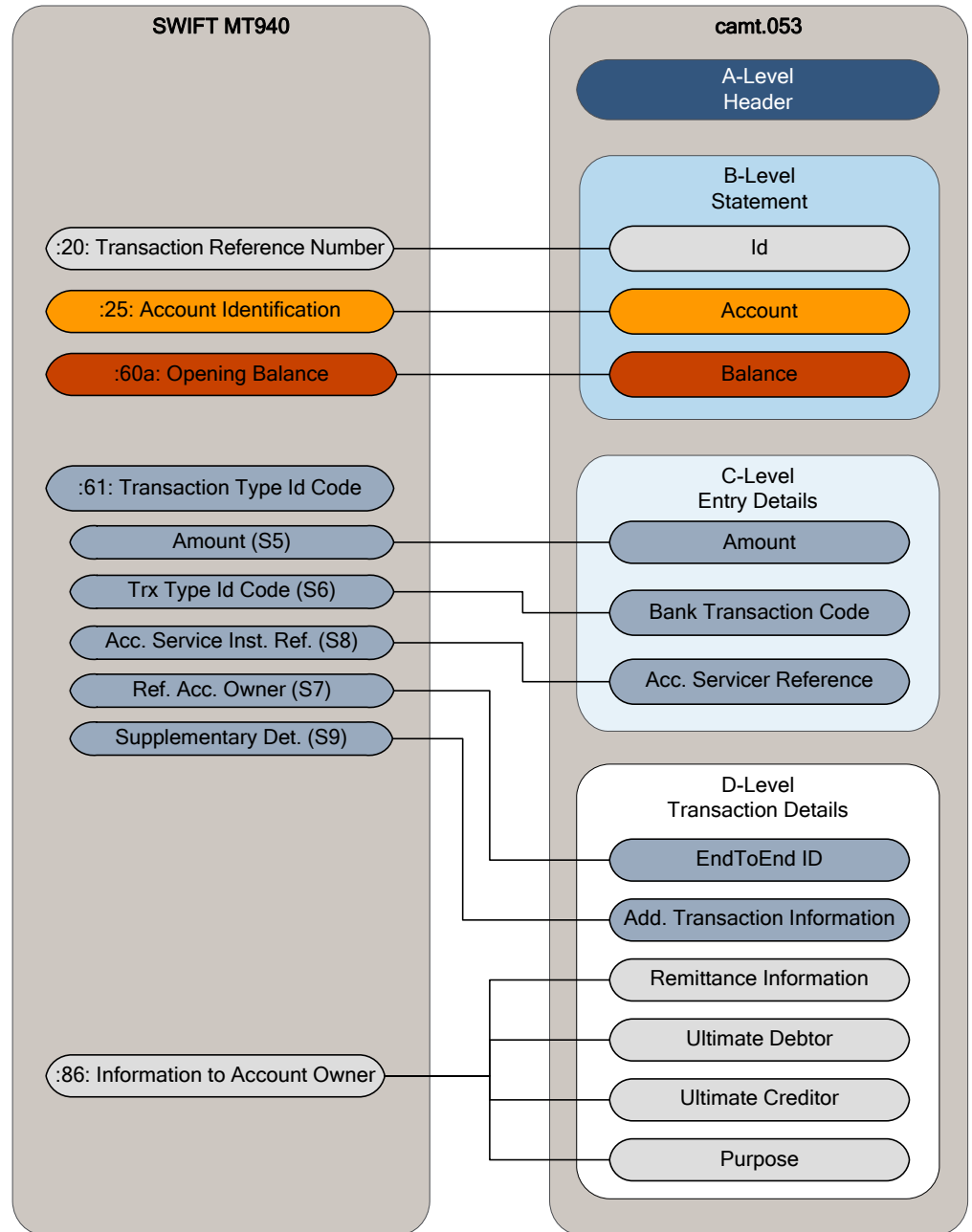
Figure 13: Summary mapping MT940 on to "camt.053"
