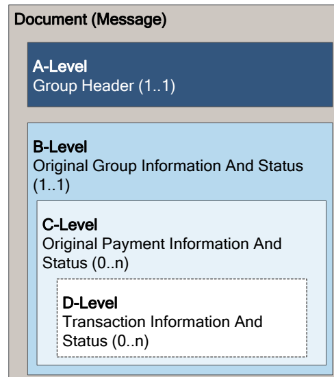
Figure 5: Message structure Payment Status Report
