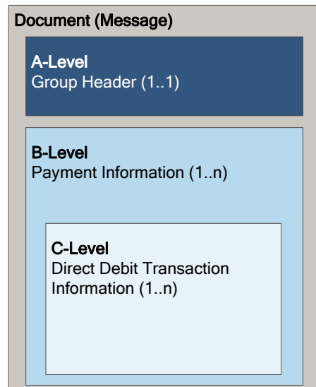
Figure 4: Message structure Customer Direct Debit Initiation
