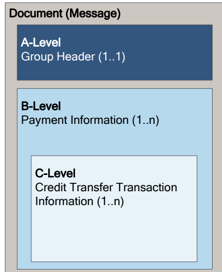
Figure 3: Message structure Customer Credit Transfer Initiation
