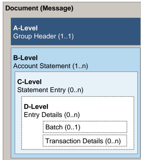
Figure 6: Message structure Cash Management messages
