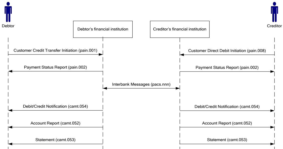
Figure 2: Payment orders under ISO 20022
