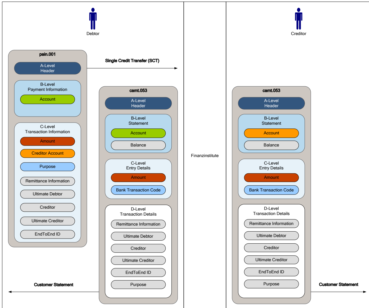
Figure 14: Interaction between "pain.001" and "camt.053"
