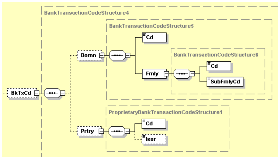
Figure 12: Bank Transaction Code
